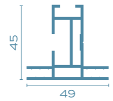
BASIC-DS-80-M.-NUT
