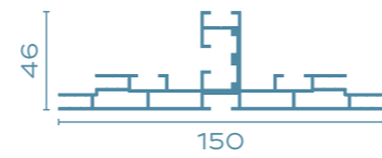
BASIC-CUBE-45°
